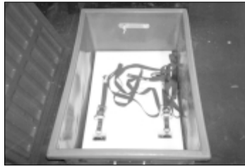
Kit installed includes foam pad, 4 pan fittings, and 2 strap and ratchet assemblies in 1" size.
