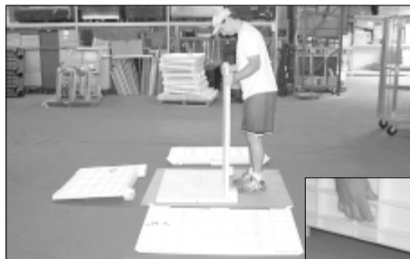
Lifting the base, insert it into the slot of this first side. Re-insert the base lock to secure this side to the base.
