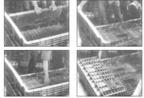
With JIT patented Slam-Latch™ system and efficient hinge design, bins can be erected or knocked down in about 5 seconds.
