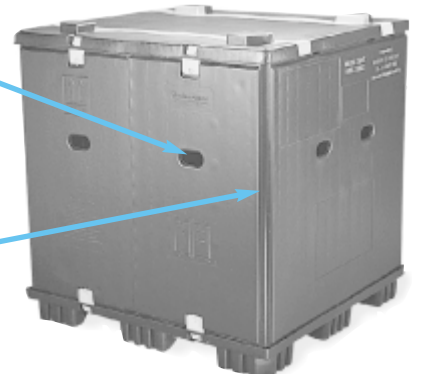
Twin Sheet Thermoformed BIG PAK for heavy duty and specialty projects
